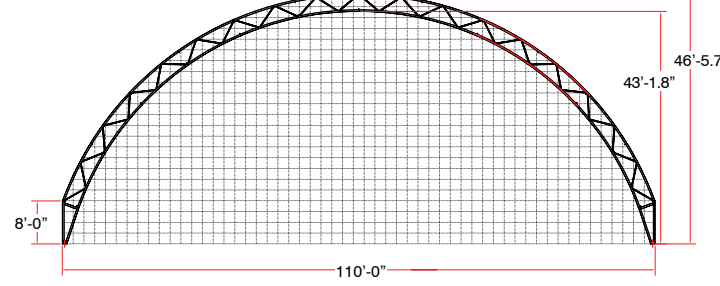
110' ARCH Requires 6 End Wall Towers
