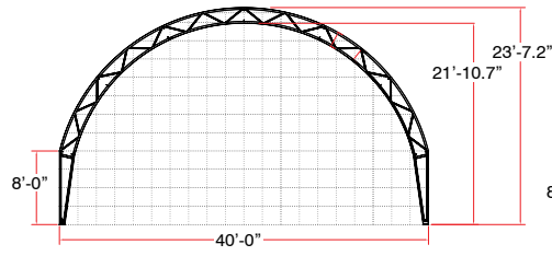
40' ARCH Requires 2 End Wall Towers
