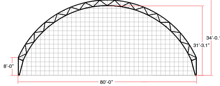
80' ARCH Requires 4 End Wall Towers
