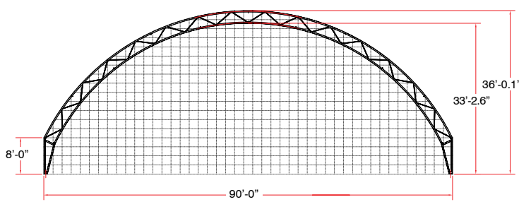
90' ARCH Requires 4 End Wall Towers
