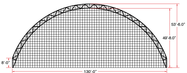
130' ARCH Requires 6 End Wall Towers
