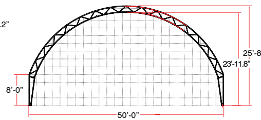
50' ARCH Requires 2 End Wall Towers
