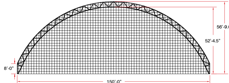
150' ARCH Requires 6 End Wall Towers
