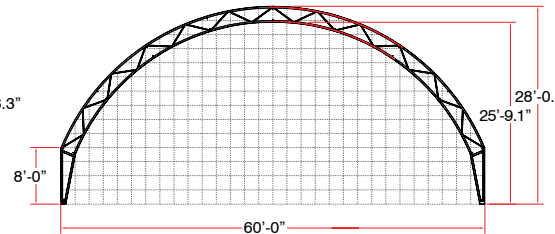
60' ARCH Requires 4 End Wall Towers
